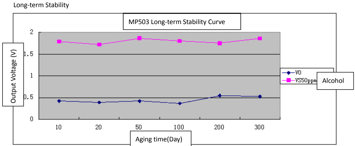
Fig7.long-term Stability of MP503
