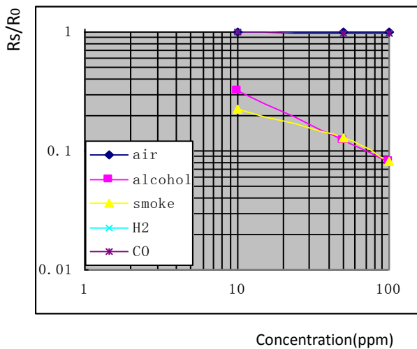
Fig3. Typical Sensitivity Curve
